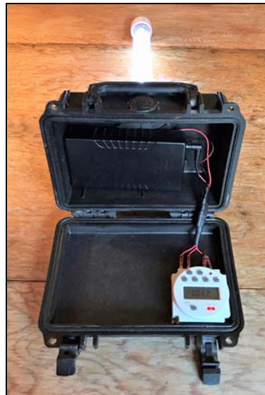
Figure 8. Fully assembled light unit with 12V lithium-ion battery and programmable timer.
