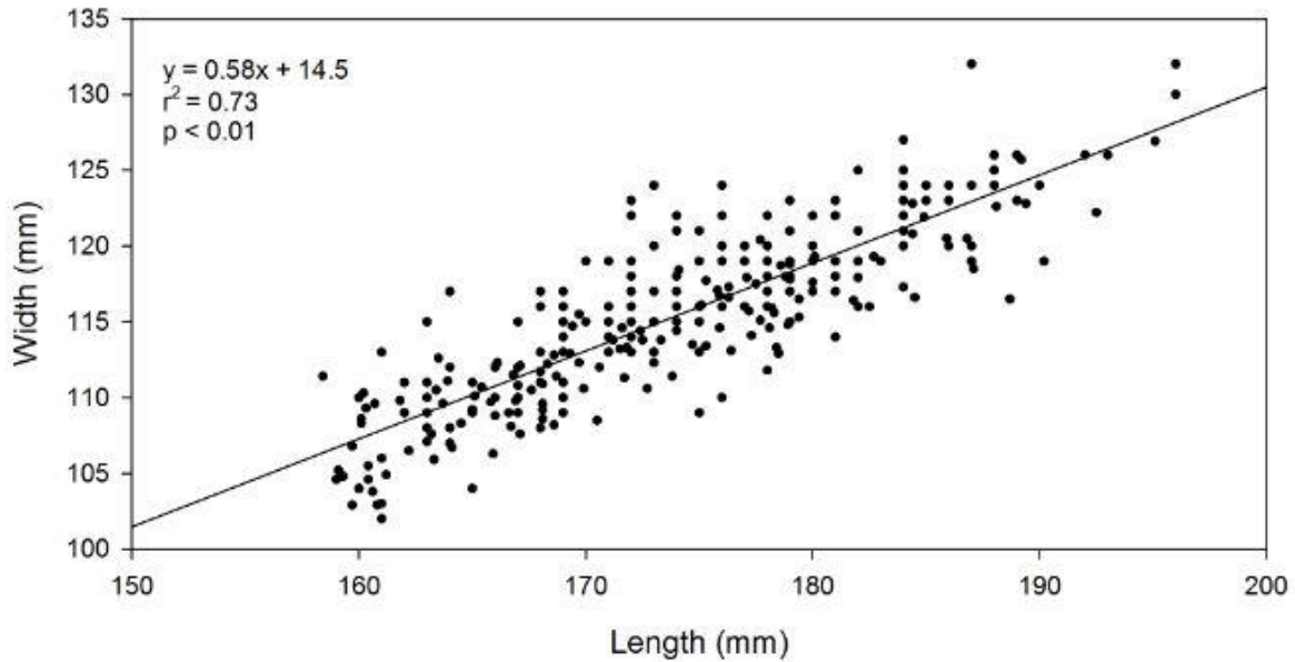
Figure 5. Length - width relationship of legal-sized male Dungeness crab, Cancer magister , in Swinomish Management Region 2 East. Solid line shows ordinary least squares regression model, n = 282.
