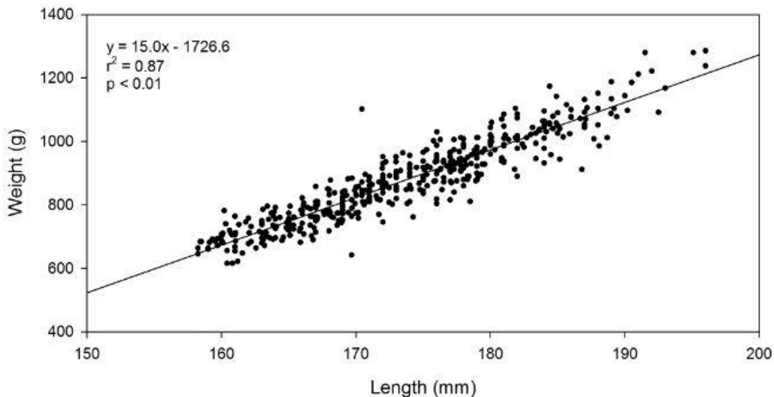
Figure 4. Length - weight relationship of legal-sized male Dungeness crab, Cancer magister , in Swinomish Management Region 2 East. Solid line shows ordinary least squares regression model, n = 446.
