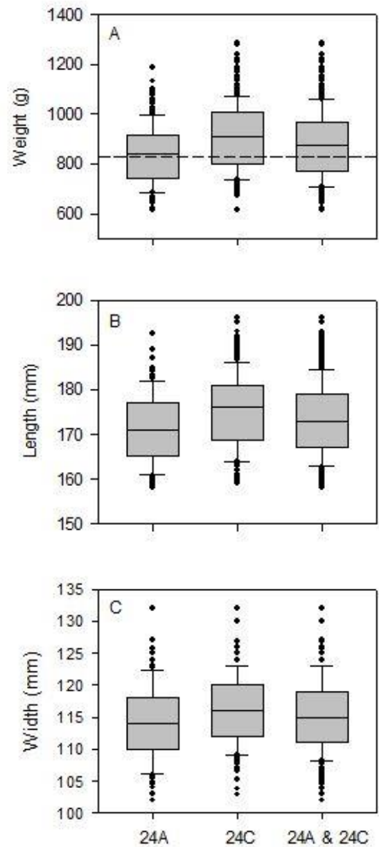
Figure 3. Box plots. A = Distribution of legal-sized male Dungeness crab, Cancer magister , weight by specific location within catch reporting areas in Swinomish Management Region 2 East (24A: n = 199; 24C: n = 247). Dashed line = 816.5 g weight used by Washington Department of Fish and Wildlife to estimate recreational harvest. B = Distribution of carapace lengths (24A: n = 199; 24C: n = 247). C = Distribution of carapace widths (24A: n = 127; 24C: n = 155). For all graphs, catch report areas 24A = Similk Bay and 24C = Crescent Harbor.
