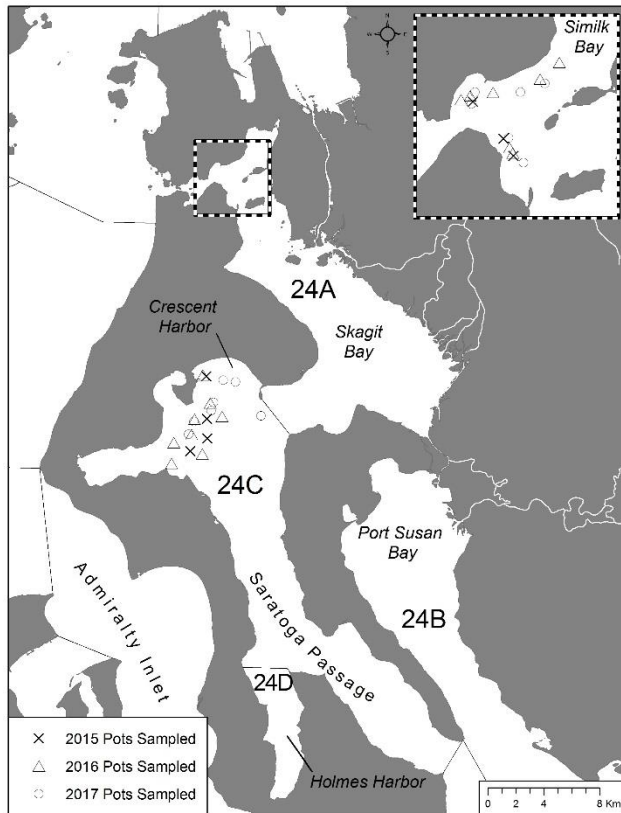
Figure 2. Crab length, width, weight sampling locations in Similk Bay and Crescent Harbor.
